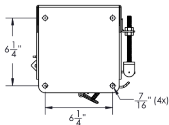
Bracket Bottom View
